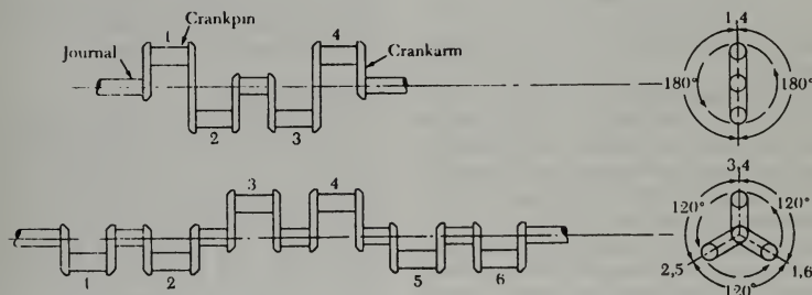
FIGURE 1-8. Solid types of crankshafts.
